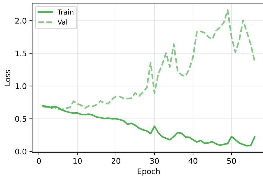
Classification Loss (BCE)
